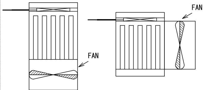
1. Air → Solid
