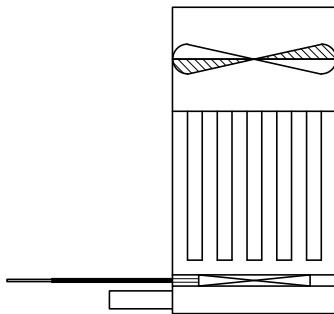
3. Liquid → Air
